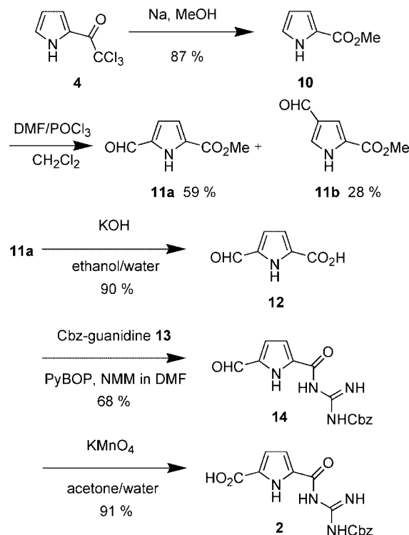
Scheme 3. Synthesis of the 5-( N -Cbz-guanidiniocarbonyl)-1 H -pyrrole-2-carboxylic acid 2 .
