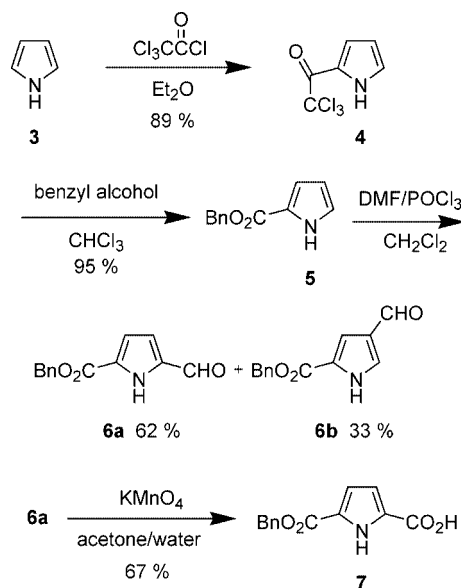
Scheme 1. Synthesis of the mono benzyl ester 7 .
