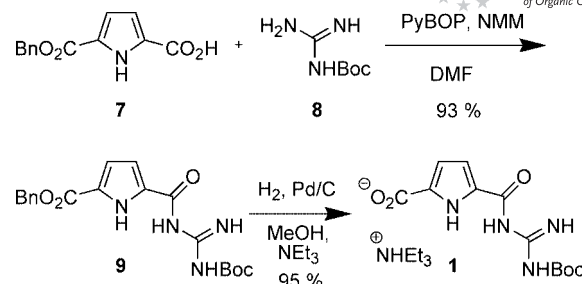
Scheme 2. Synthesis of the 5-( N -Boc-guanidiniocarbonyl)-1 H -pyrrole-2-carboxylic acid ( 1 ).
